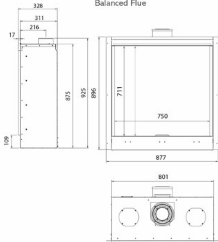
Balanced Flue
