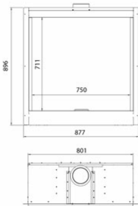
Conventional Flue
